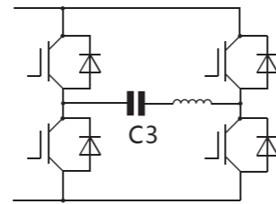
Resonance Capacitors(C3)
